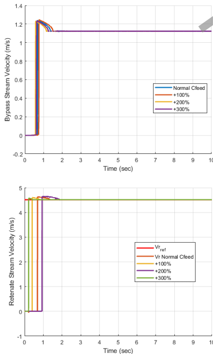
Figure 3. The performance of the super twisting sliding model controller in dealing with disturbances in water salinity
