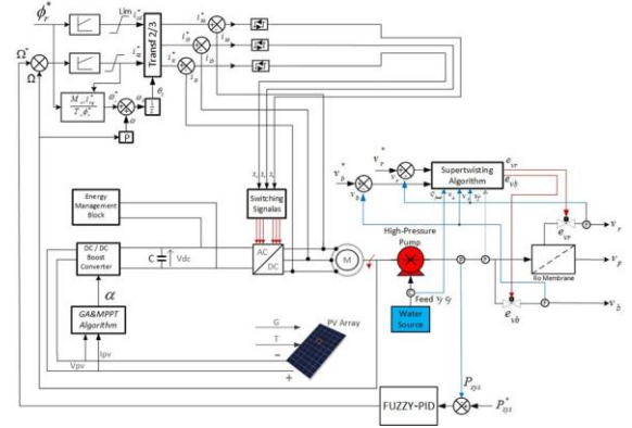
Figure 1. Combination of reverse osmosis desalination system and photovoltaic system
