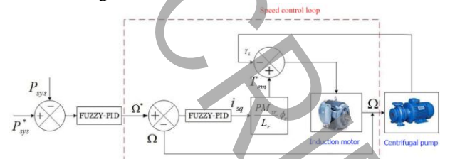
Figure 2. Motor-pump set with fuzzy PID control algorithm
