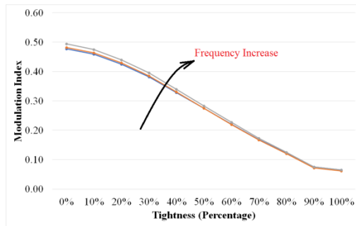
Fig. 7. The effect of ultrasonic frequency excitation on modulation indices at sensor-actuator location 45 (Numerical analysis)
