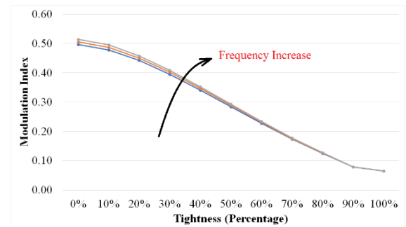
Fig. 6. The effect of ultrasonic frequency excitation on modulation indices at sensor-actuator location 45 (Experimental analysis)
