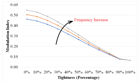
Fig. 4. The effect of the vibrational excitation frequency on modulation indexes in sensor-actuator position 45 (Experimental analysis)
