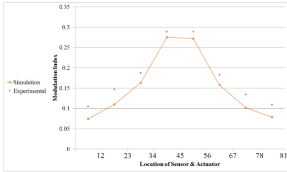
Fig. 1. Modulation index at different sensor-actuator positions at 50% looseness
