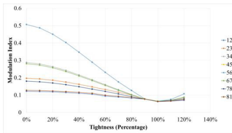
Fig. 2. The effect of excessive increase of torque on modulation indexes in different sensor-actuator locations (Experimental analysis)
