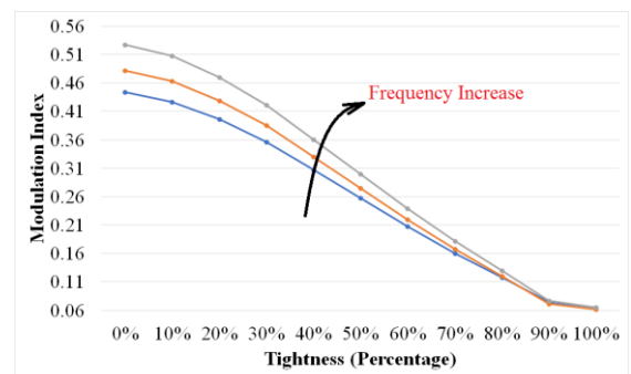
Fig. 5 The effect of the vibrational excitation frequency on modulation indexes in sensor-actuator position 45 (Numerical analysis)
