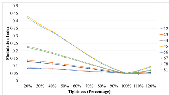
Fig. 3. The effect of excessive increase of torque on modulation indexes in different sensor-actuator locations (Numerical analysis)
