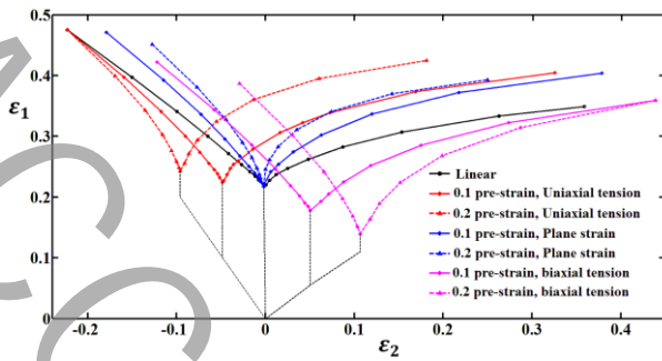
Figure1. The FLCs based on different pre-strains along different direction
