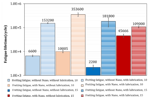
Figure 2: The effect of the lubricant addition on the FF lifetime of the aluminum alloy
