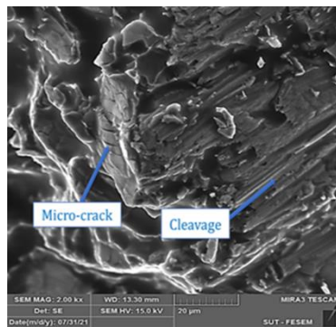
Figure 3: FESEM images from the fracture surface of the sample with nano-particles and the lubrication at 15 N
