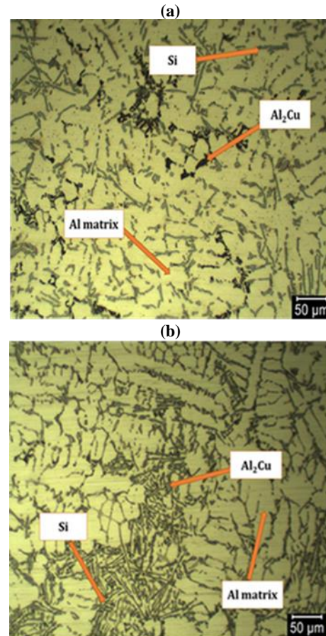
Figure 1: Aluminum alloy microstructures: (a) without nano-particles and (b) with nano-particles
