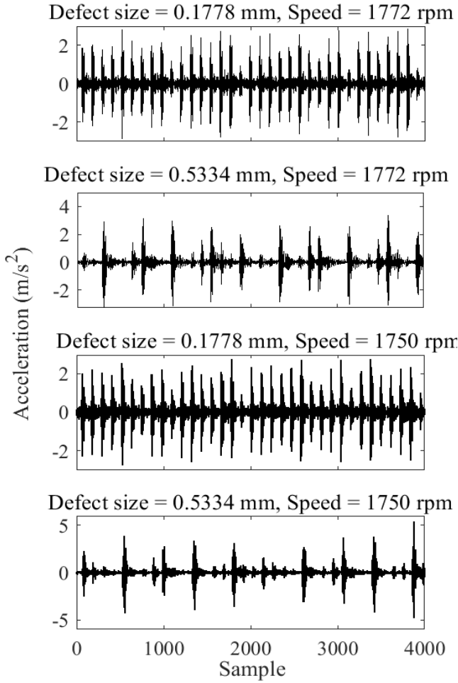
Fig. 1. The vibration signals corresponding to the defective outer ring
