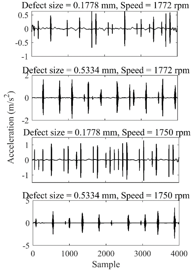
Fig. 2. Denoised signals corresponding to the defective outer ring
