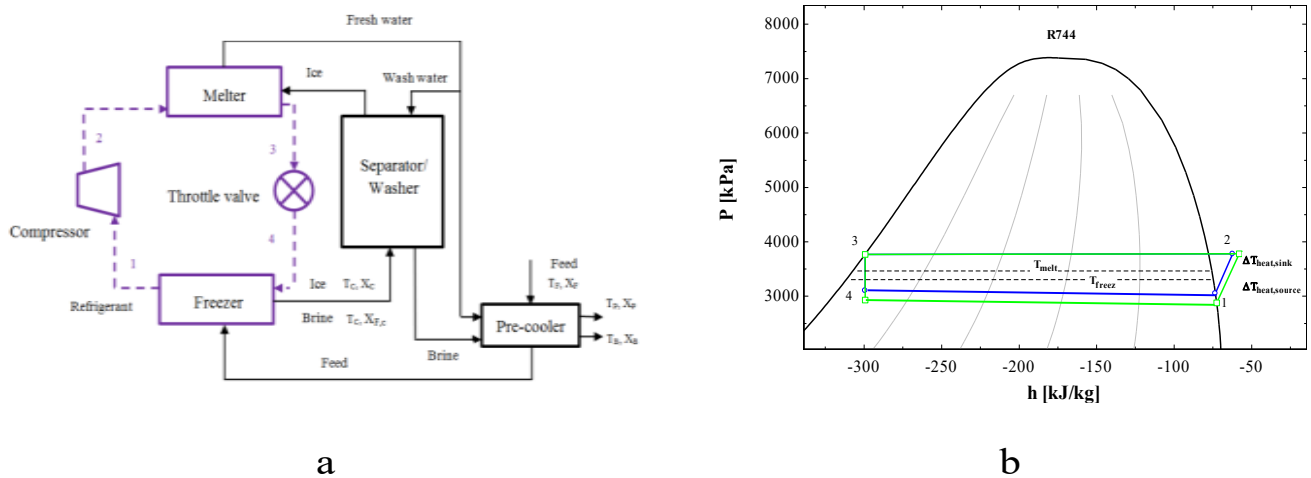
Fig. 1. a) Schematic of the combined FD system and a CO 2 refrigeration system, b) p-h diagram of CO 2 refrigeration system
